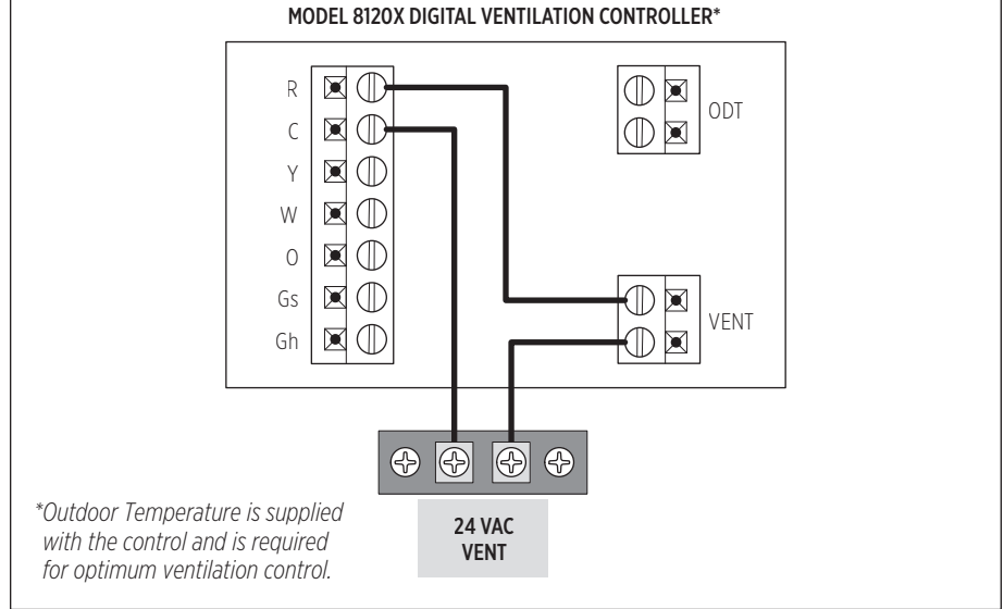
FIGURE 4 – WIRING TO MODEL 8142NC FRESH AIR VENTILATOR
