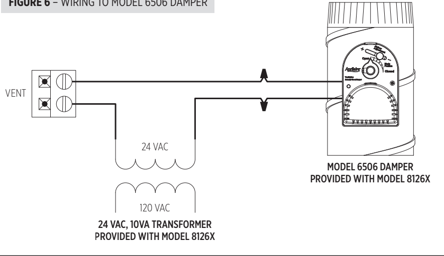
FIGURE 6 – WIRING TO MODEL 6506 DAMPER
