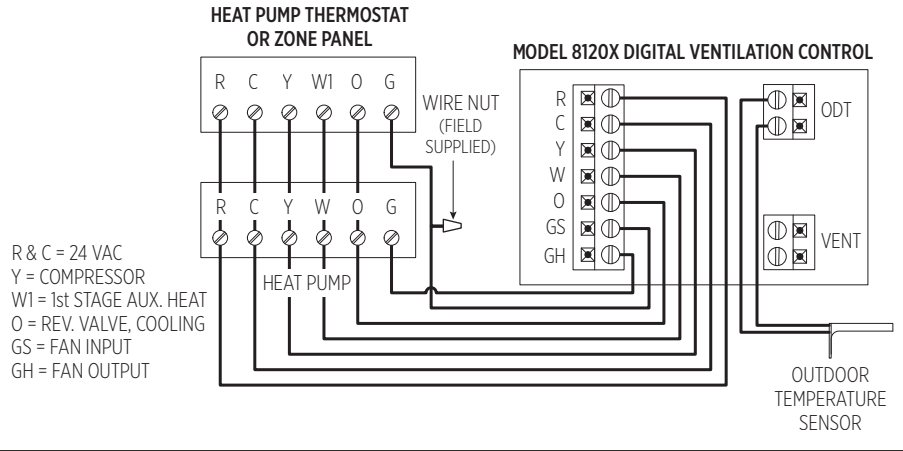
FIGURE 2 – WIRING TO HEAT PUMP
