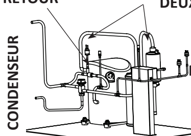
CLAPET ANTI-RETOUR
