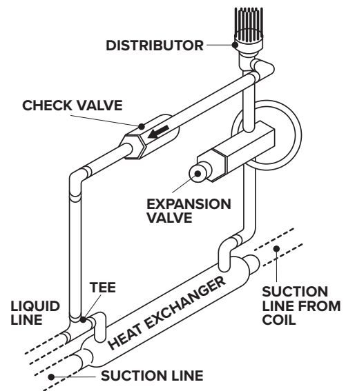
FIGURE 2. Typical Liquid Line Bypass Kit
