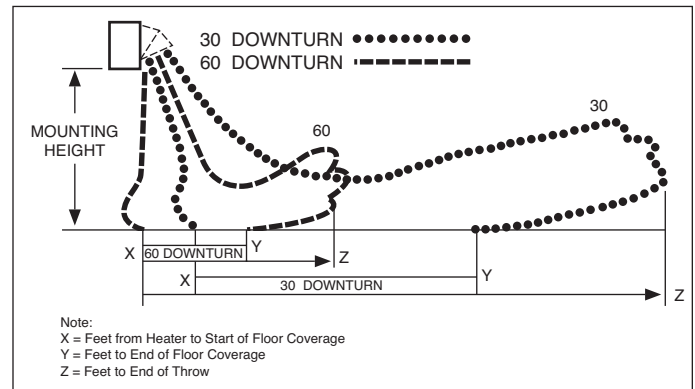
Figure 16.2 - 30° and 60° Throw/Floor Coverage
