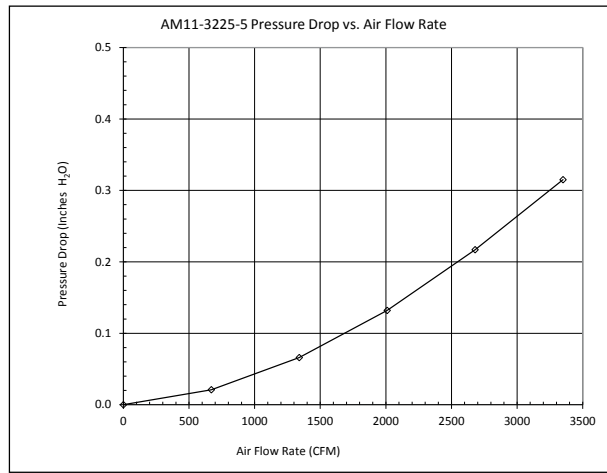
AM11-3225-5 Pressure Drop vs. Air Flow Rate
