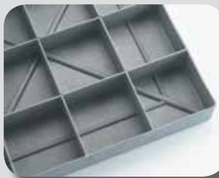
The bottom of a 3" E Lite® pad shows ribbing plus additional surface support.
