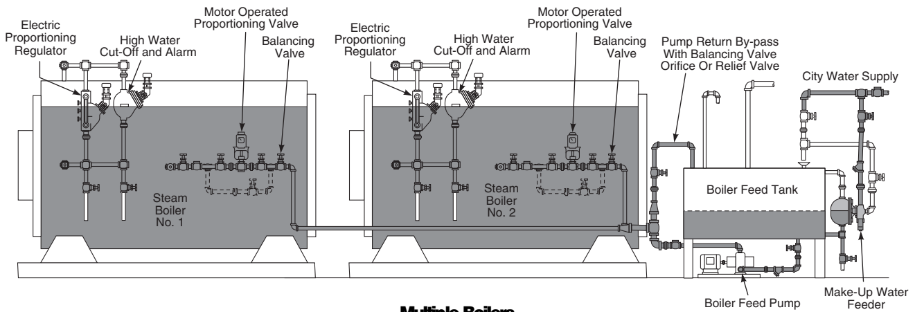
Multiple Boilers Boiler Feed Pump, Electric Proportioning Regulators and Motorized Valves
