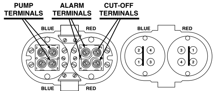
At Normal Operating Level Boiler feed pump off— burner on—alarm off.
