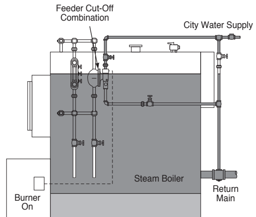
Large Boilers
