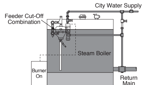
Normal Operation
