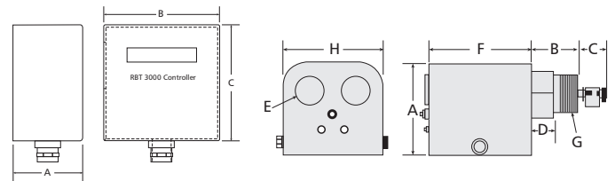
Control Box
