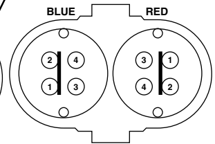
At Normal Operating Level Boiler feed pump off— burner on—alarm off.
