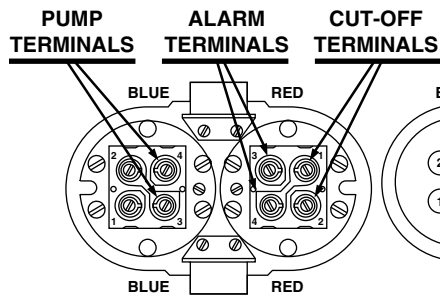
No. 5 Switch Used on 93, 193, 94 and 194 Series.
