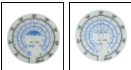
Actual gauge tipped at two different angles.
