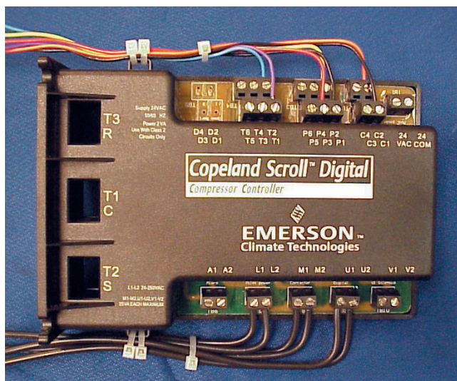
Figure 1 – Digital Compressor Controller 543-0024-00, -01
