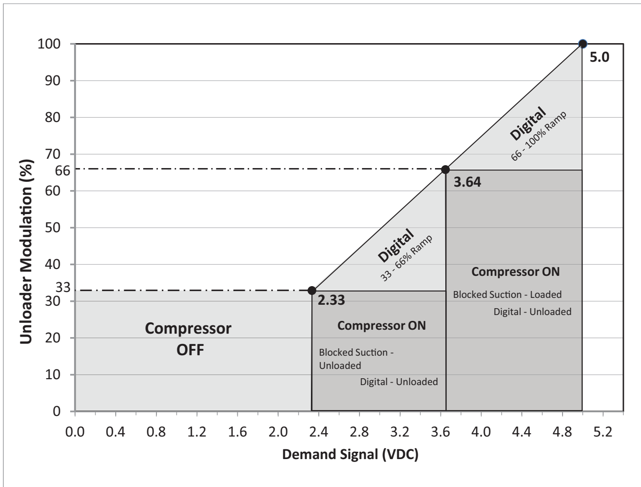
Figure 6 Demand Signal vs. Modulation Graph (P/N 543-0194-00)
