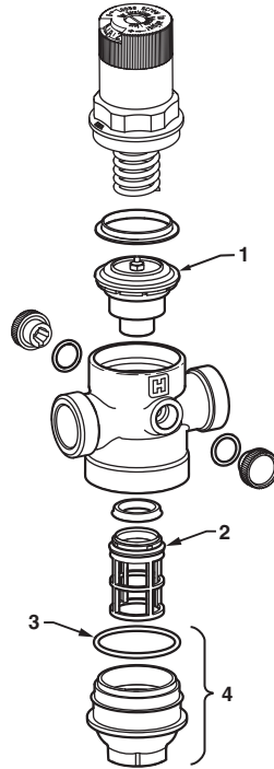
Fig. 5. Replacement Parts.
